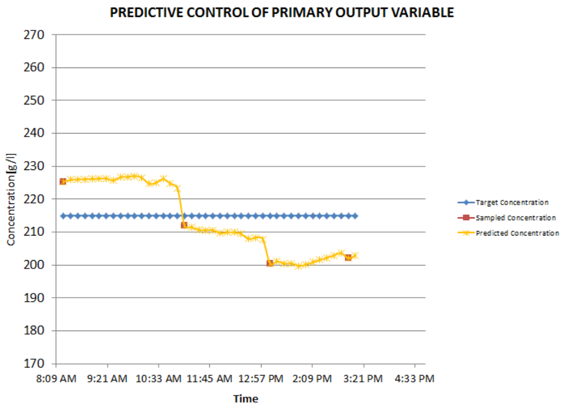
Figure 40. Predicted Concentration during Predictive Control Operation of the first test for Phase 4.
