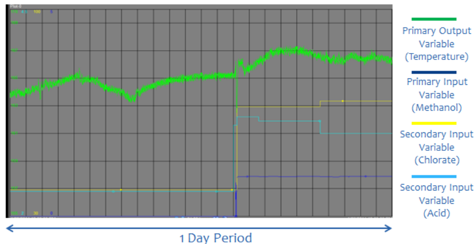
Figure 30. Start Up Operation of a Chlorine Dioxide Generator.
