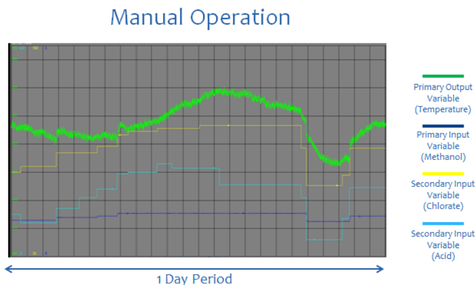
Figure 35. Temperature during Manual Operation of the day before testing for Phase 2. This image shows manual operation of the system the day before testing of stabilizing procedures.
