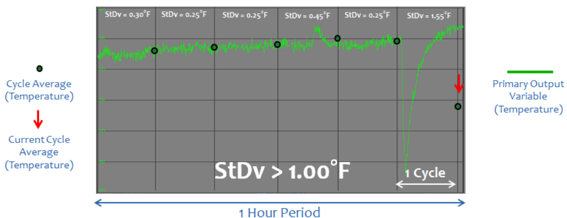
Figure 19. Error-in-Temperature-Data Pattern for a Chlorine Dioxide Generator.
