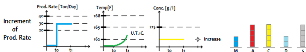
Figure 24. Predictive Control of Outputs: Increment of Production Rate.
