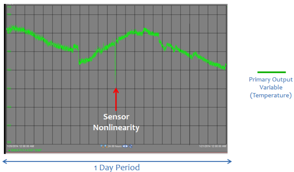
Figure 18. Sensor Nonlinearity of a Temperature Trend.
