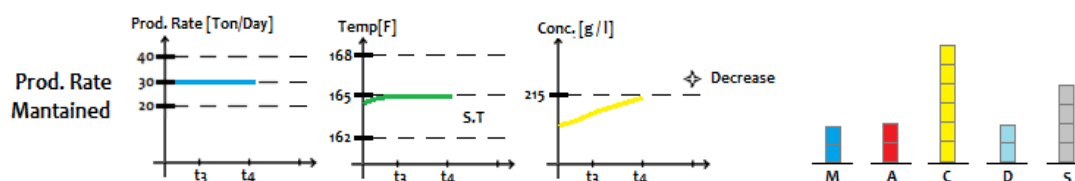
Figure 26. Predictive Control of Outputs: Production Maintained while Correcting Concentration. This image shows the output and the input variables when the production rate on a chlorine dioxide generator is maintained while the predictive control attempts to bring the concentration to its target.
