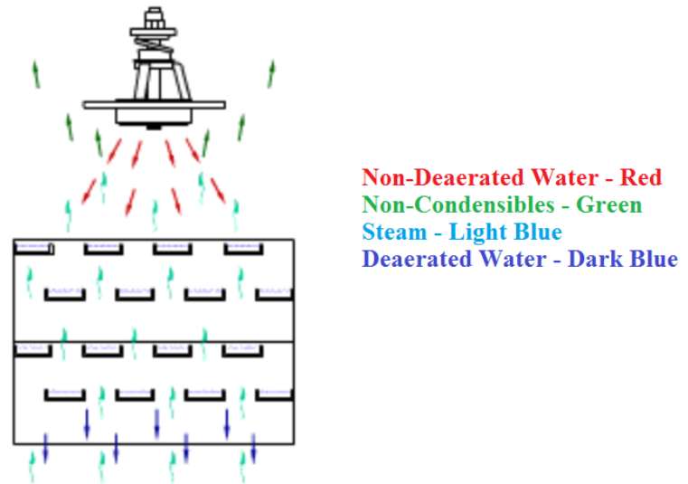
Figure 8. The Deaerator Principle for removing gas particles from a substance.
