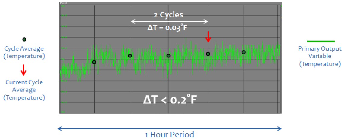
Figure 13. Stable-Temperature Pattern for a Chlorine Dioxide Generator.
