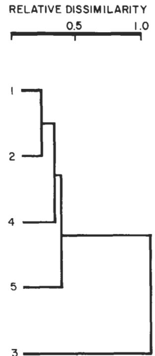
Figure 4. Clustering of combined collection periods by station using Bray-Curtis dissimilarity index and flexible sorting.
