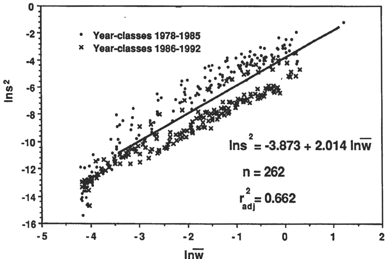
Figure 2. Relationship between natural logarithms of variances and arithmetic means ( lns^2 and ln\bar{w} , respectively) of weight ( w , kg) in samples of captive-reared Kemp's ridleys ( Lepidochelys kempii ) containing 25 or more turtles at age t . The straight line was fitted to 262 data points representing turtles 0.17 to 1.22 yr of age, but the scatter also included 86 data points for turtles < 0.17 yr old.
