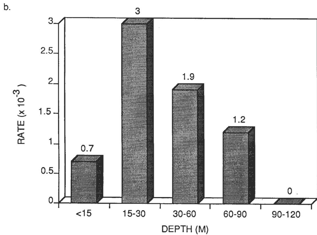
Figure 3. a. Aerial observation rates (individual sea turtles per hour \times 10^{-3} ) by depth zone, and b. Surface observation rates (individual sea turtles per hour \times 10^{-3} ) by depth zone.
