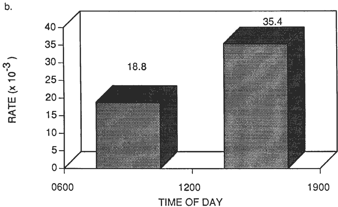
Figure 4. a. Rate (sightings per monitoring hour \times 10^{-3} ) of sea turtle sightings from surface surveys by time of day, and b. Rate (sightings per monitoring hour \times 10^{-3} ) of sea turtle sightings from aerial surveys by time of day. Aerial surveys were only conducted during daylight hours.
