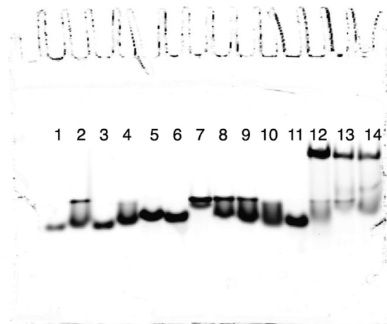
Fig. 2. Comparison of multi-DNAs vs. J1, 4WJ:PNA 1 and b4WJ:PNA 1 .
