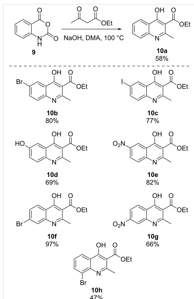
Scheme 4: Substituted 2-methyl-4-hydroxyquinolines from isatoic anhydrides and ethyl acetoacetate.
