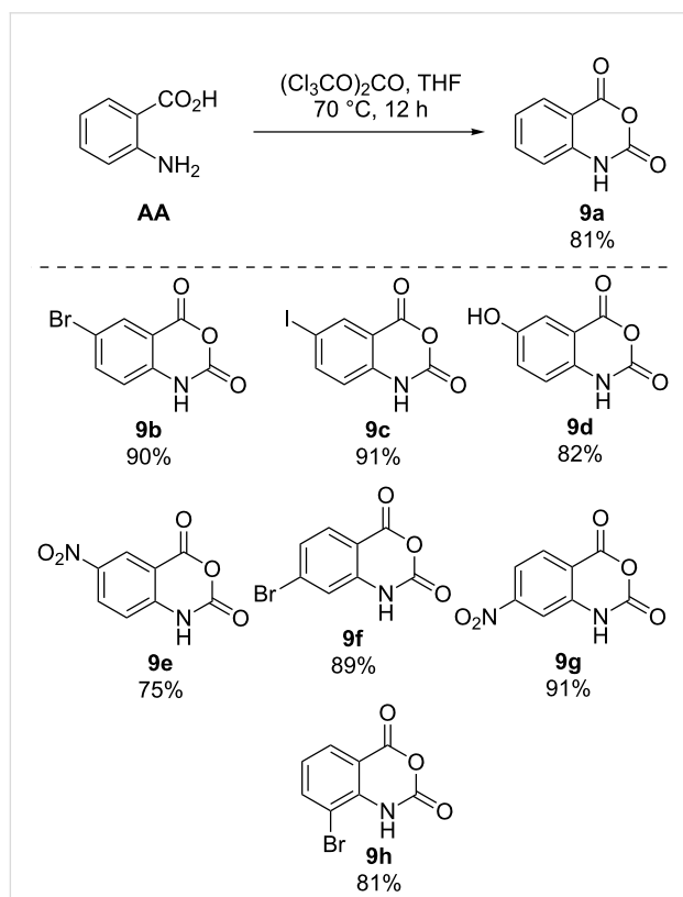
Scheme 3: Isatoic anhydrides from anthranilic acids with triphosgene.
