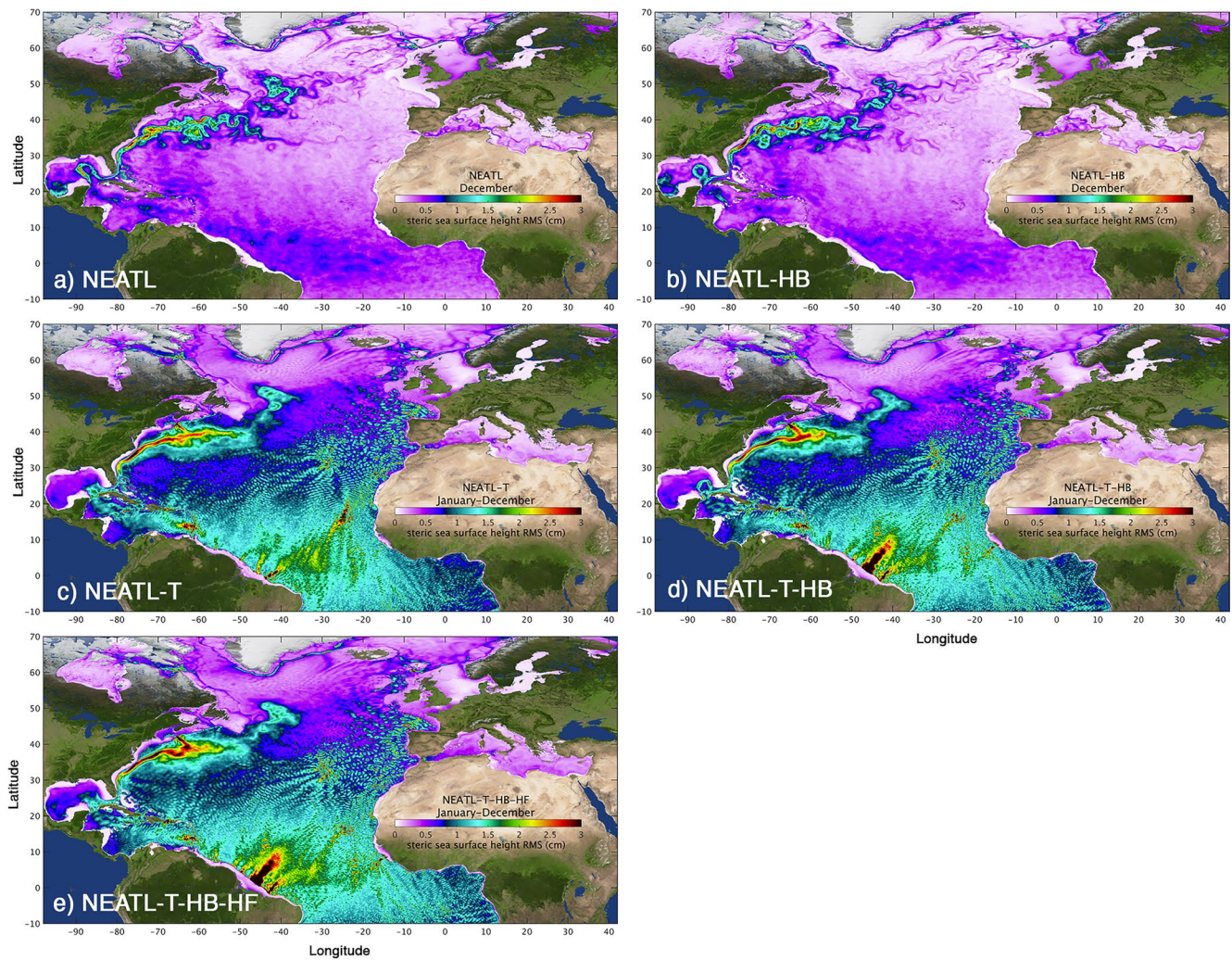
Figure 2. Standard deviation value of the modeled high-frequency steric sea surface height (SSH, in cm) variability in five 1/50° Atlantic simulations that are summarized in Table 1: (a) NEATL, (b) NEATL-HB, (c) NEATL-T, (d) NEATL-T-HB, and (e) NEATL-T-HB-HF. The standard deviation is calculated from the hourly snapshots of the SSH within a day and averaged over 1 month for experiments a-b and over 1 year for experiments (c-e) (to reduce spatial noise).
