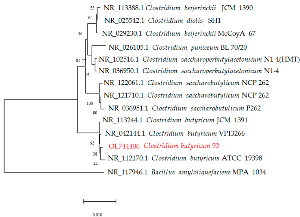
Figure 1. Phylogenetic tree, built using closely related species by the method of joining neighbors (using MEGAX software). The initial values (%) are set in the nodes obtained by repeating the analysis 1000 times. The size of the scale characterizes 0.01 nucleotide substitutions for each nucleotide position. The Bacillus amyloliquefaciens MPA 1034 demonstrated as an outgroup for rooting a phylogenetic tree.
