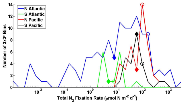
Figure 10. Histograms of depth-integrated total N_2 fixation rates (after binned on 3^\circ \times 3^\circ grid) in North Atlantic (blue), South Atlantic (green), North Pacific (red) and South Pacific (black). For each basin, filled diamond and empty circle mark the location of the geometric mean and the arithmetic mean, respectively.
