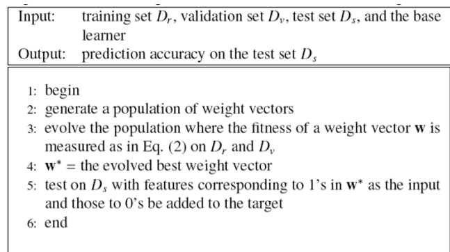
Figure 5 Genetic algorithm based multi-task learning (GA-MTL)
