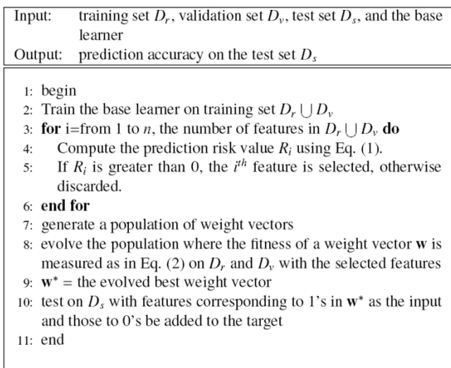
Figure 6 GA-MTL with irrelevant feature removed (GA-MTL-IR)
