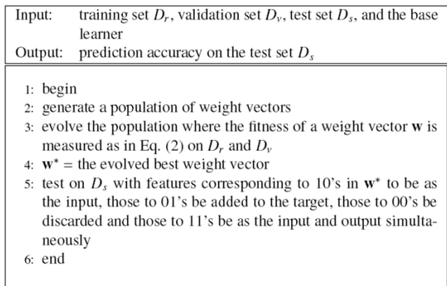
Figure 7 Enhanced version of GA-MTL (e-GA-MTL)
